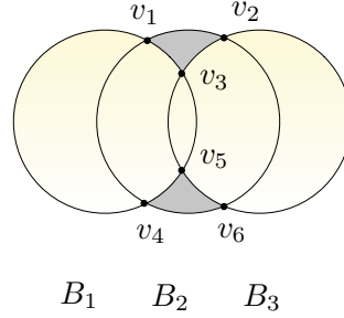
Fig. 2. A planar (multi)graph P_I formed from unit disk graph G with three vertices B_1, B_2 , and B_3 . The vertex set of P_I is \{v_1, \dots, v_6\} . It has 7 regions. For example, for region \mathcal{R}_1 bounded by v_1, v_3, v_5, v_4 , we have \mathcal{V}(\mathcal{R}_1) = \{B_1, B_2\} . For region \mathcal{R}_2 bounded by v_1, v_2, v_3 and region \mathcal{R}_3 bounded by v_4, v_5, v_6 , we have \mathcal{V}(\mathcal{R}_2) = \mathcal{V}(\mathcal{R}_3) = \{B_2\} . The outer face of P_I is not a region.
