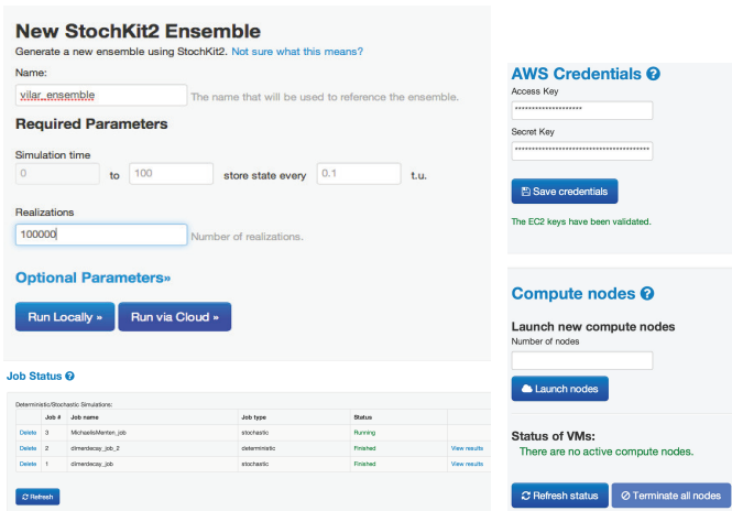
Figure 4. StochSS Web UI constructed using CLOUDRUNNER.
