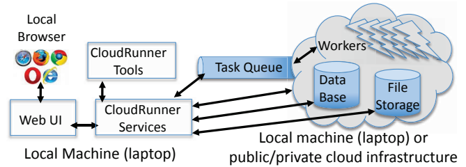
Figure 1. CLOUDRUNNER system overview.
