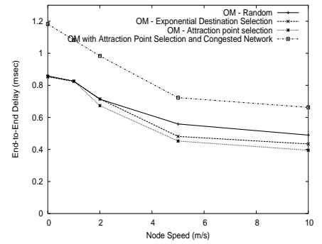
Figure 12: End-to-End Latency.
