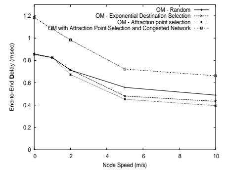
Figure 12: End-to-End Latency.
