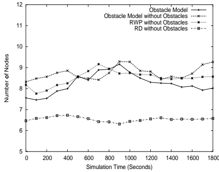
Figure 3: Node Density.
