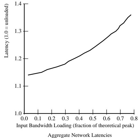
The graph shows latency versus network loading for randomly distributed, 20-byte message traffic on a 3-stage network constructed from 8-bit wide, radix-4 METRO routers. This simulation models a parallelism limited case where processors stall waiting for message completion. The first two network stages are configured in dilation-2 mode, while the last stage is configured in dilation-1 mode. Like the network shown in Figure 1, each endpoint has two connections entering and leaving the network. Each endpoint was restricted to only use one of its entering network ports at a time, but can handle simultaneous traffic on both network output ports. The unloaded message latency is 28 clock cycles from message injection to acknowledgment receipt.
