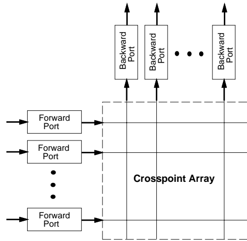
The basic router has i forward ports and o = r \cdot d backward ports. Any forward port can be connected through the crosspoint array to any backward port. The arrows indicate the initial direction of data flow.
